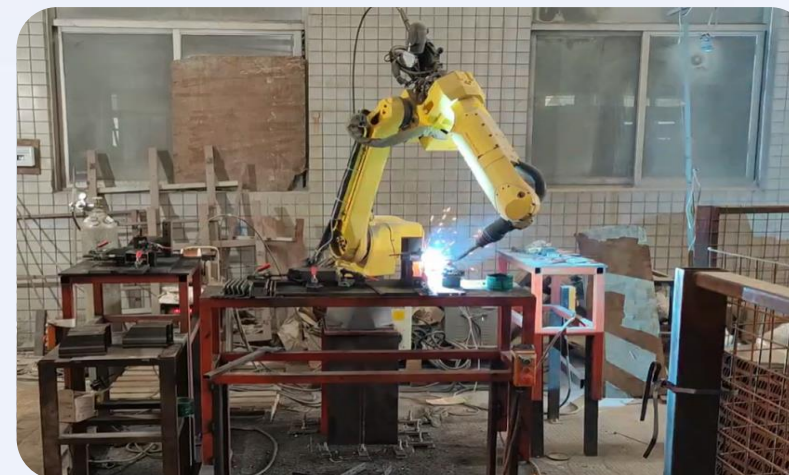
Welding Manipulator
