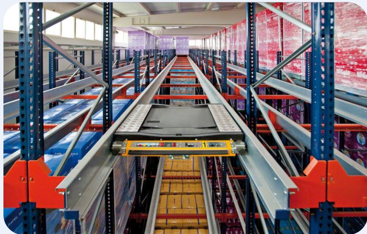
Drive-in Rack
